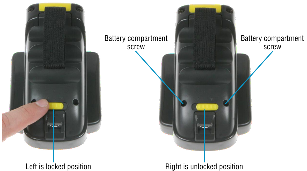
FIGURE 2: Unlock Battery Compartment
